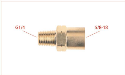
Part No. CN-AW-15 Description Water Hose Coupler 5/8-18 LH-G1/4 Male Pipe
