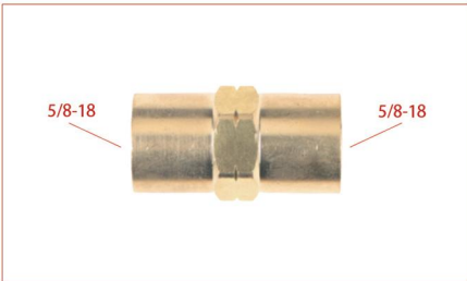
Part No. CN-11N17 Description Gas Hose Coupler 5/8-18
