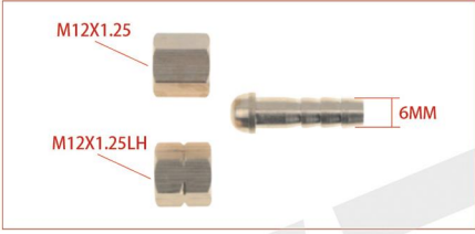
Part No. CN-NUTM12X1.25 Description Nut M12X1.25
