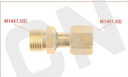
Part No. CN-M14X1.5(E)-M16X1.5(I) Description Power Cable Adapter
