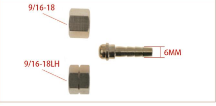
Part No. CN-NUT9/16-18 Description Nut 9/16-18
