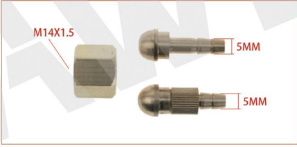
Part No. CN-NUTM14X1.5 Description NutM14X1.5
