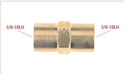
Part No. CN-11N18 Description Water Hose Coupler 5/8-18 LH
