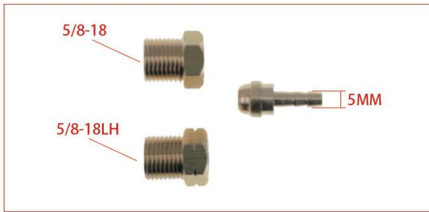
Part No. CN-136Z08 Description Nut 5/8-18
