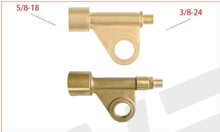
Part No. CN-53N43 Description Power Cable Adapter Sketch Torch Series:24
