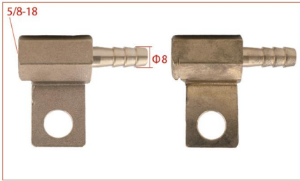
Part No. CN-BRA5818 Description Power Cable Adapter Sketch Torch Series:26
